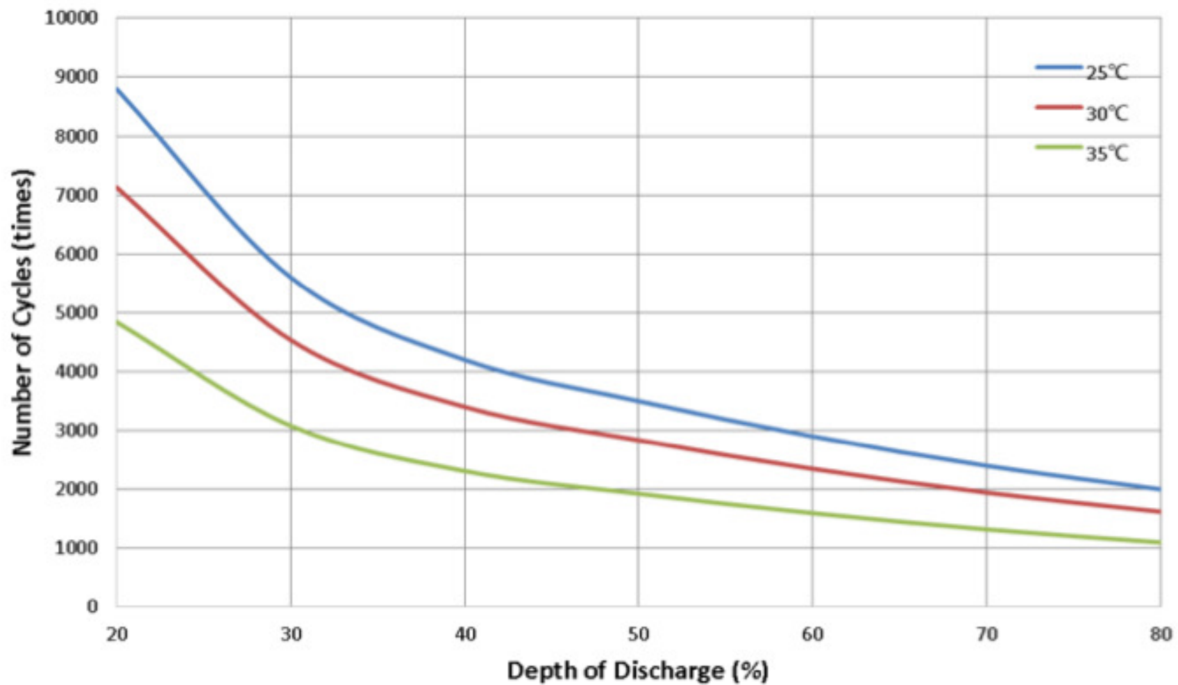
HEL-C battery cycle life at different temperature and depth of discharge
